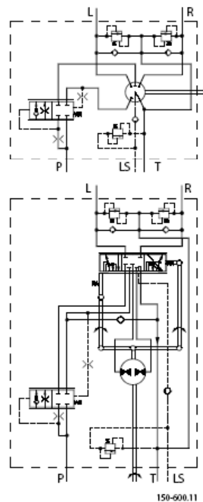
OSPQ LS (OLS) Load sensing dynamic non-reaction
