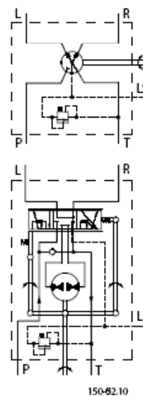
OSPCX LS Load sensing dynamic
