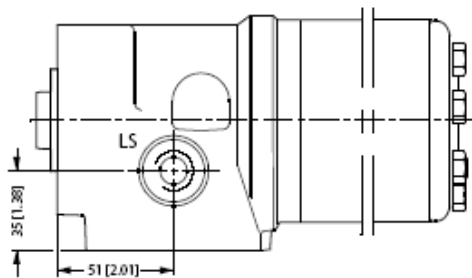
OSPL LS with relief valve
