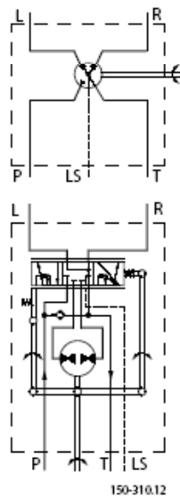
OSPBX LS, OSPLX LS Load sensing static
