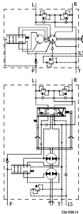
OSPD LS (OLS) Load sensing dynamic non-reaction
