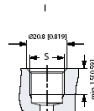
I: UNF ports w. O-ring 150-609.10 chamfer (P, T, L, R) S: ISO 11926-1 - ¾-16UNF O-ring boss port
