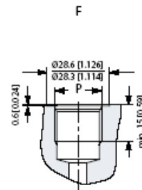
F: Metric ports w. spot face and O-ring chamfer (P, T, L, R) P: ISO 6149-1 - M18 x 1.5
