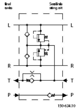
OVPL, 4 ports and backpressure valve with by-pass
