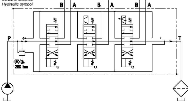
Schema idraulico Hydraulic symbol
