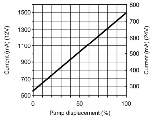
Electrovalve current vs Displacement
