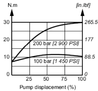
Control shaft torque at 1500 rpm
