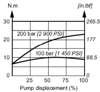
Control shaft torque at 3000 rpm
