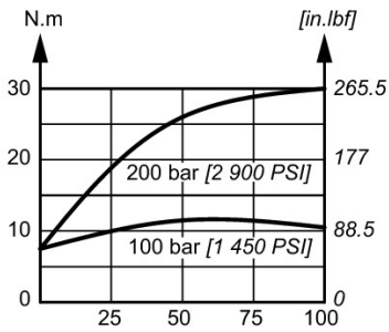
Control shaft torque at 1500 rpm
