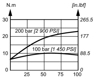
Control shaft torque at 3000 rpm
