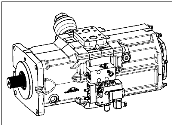
Double pump with SAE J744 flange
