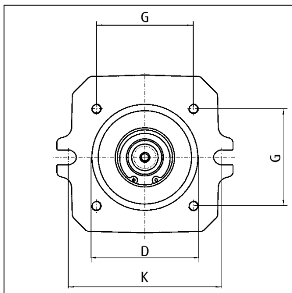
2-hole flange with 4 additional threaded holes
