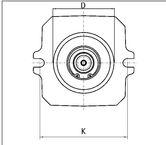
2-hole flange with 4 additional threaded holes
