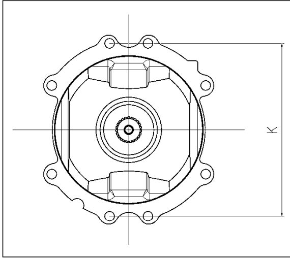
Plug-in flange
