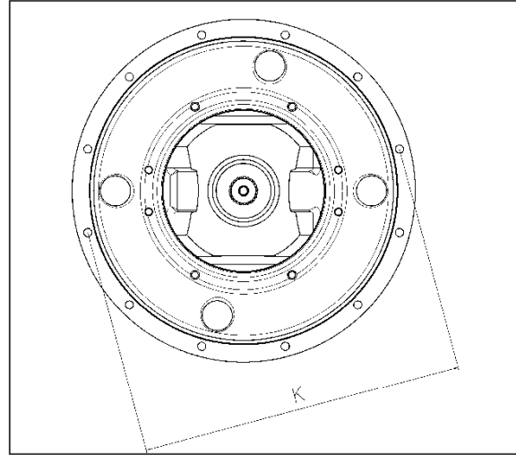
SAE bell housing
