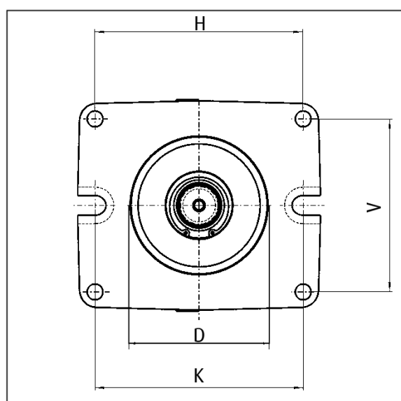
2-hole flange with 4 additional bolt holes
