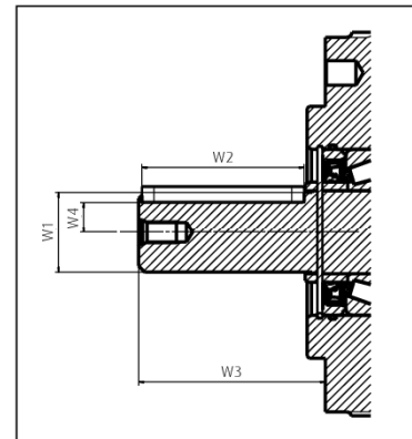
Mounting flange
