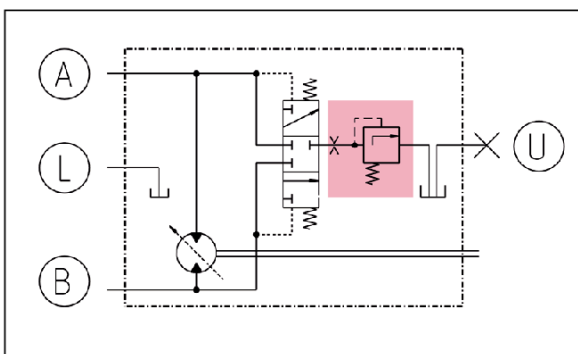
Purge valve 3. Restricted
