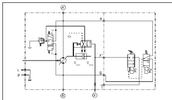
EH1P. Case pressure as reference, «Bleed» regulation
