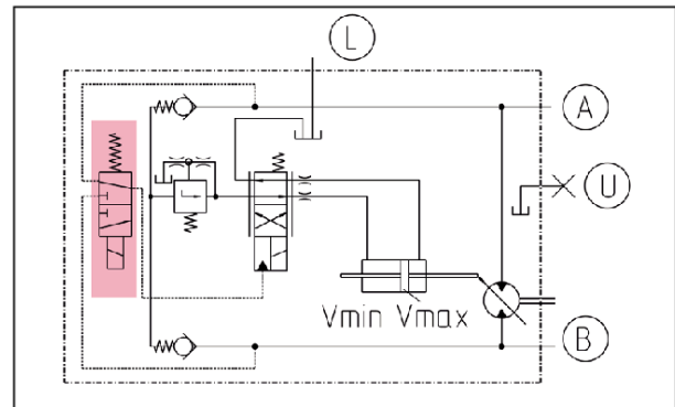
With signal selection for pressure regulator
