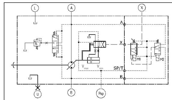
EH1P-CA. Feed pressure as reference, «Non-Bleed» regulation
